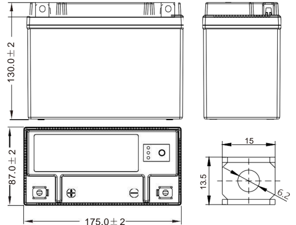
Dimensions (mm)
