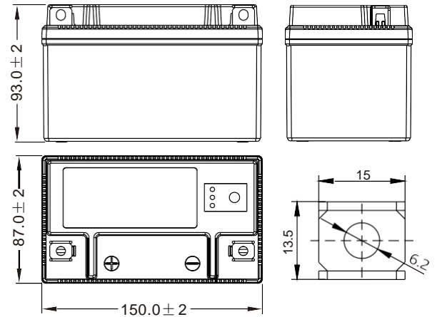
Dimensions (mm)
