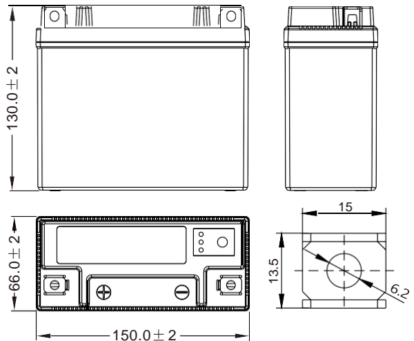
Dimensions (mm)
