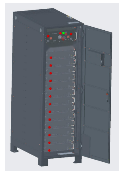
Rack BU665V200(S) BU665V200--without SBMS, BU665V200(S)-with SBMS
