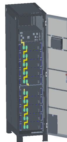
Rack BU512V100(S) BU512V100--without SBMS, BU512V100(S)-with SBMS
