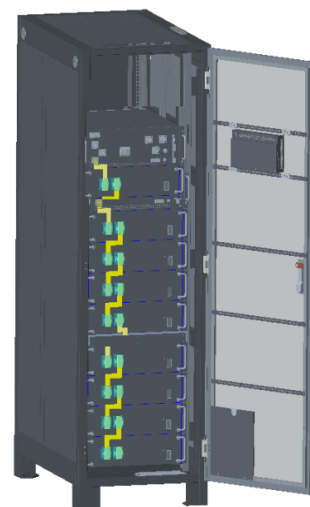
Rack BU460V100(S) BU460V100--without SBMS, BU460V100(S)-with SBMS
