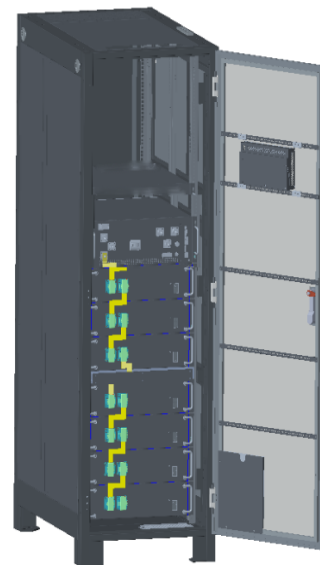
Rack BU358V100(S) BU358V100--without SBMS, BU358V100(S)-with SBMS
